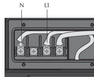
Chauffe-eau 120 VAC (1 KW)
