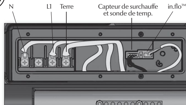
Chauffe-eau 120 VAC (1 KW)
